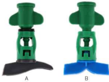
Spinner micro sprinkler (φ7.5mm)
